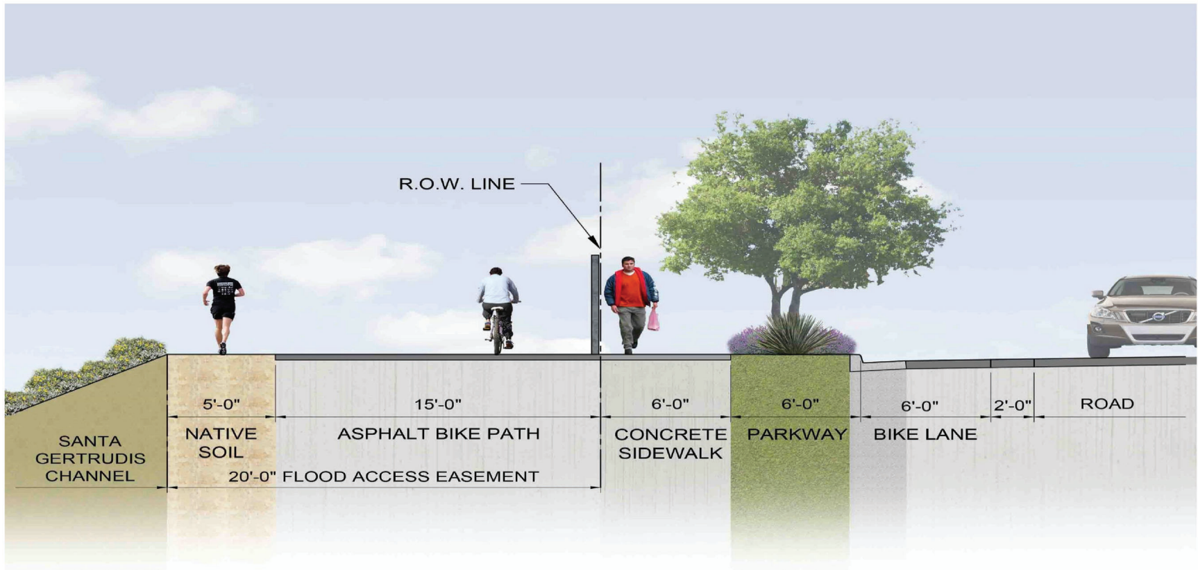
TRAIL TYPE H - NICOLAS ROAD: CALLE GIRASOL TO JOSEPH RD. (15' ASPHALT TRAIL ALONG CHANNEL)
