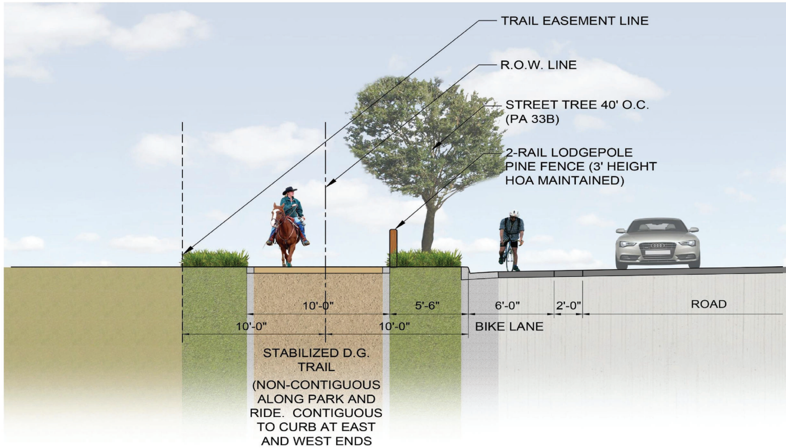
TRAIL TYPE G - NICOLAS ROAD: BUTTERFIELD STAGE RD. TO W. PROJECT BOUNDARY (10' D.G. TRAIL)
